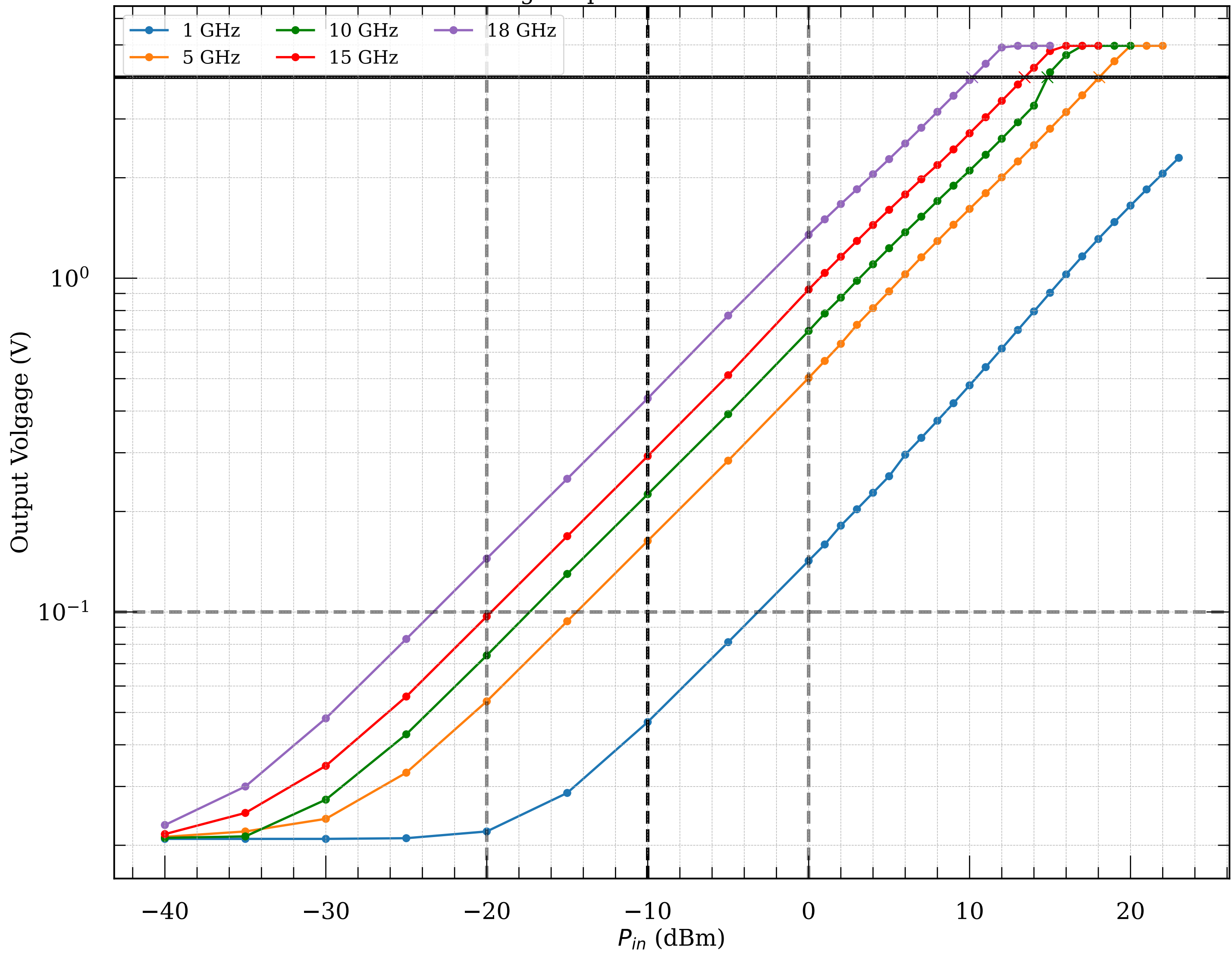
Measured voltage-to-power curve of detector module034
